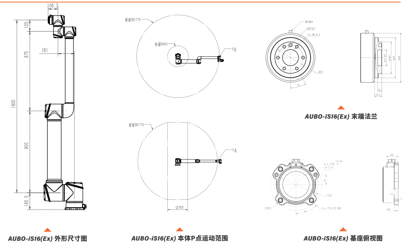
Dimension Drawings
